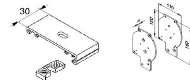
Bracket Detail
