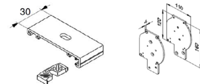
Bracket Detail
