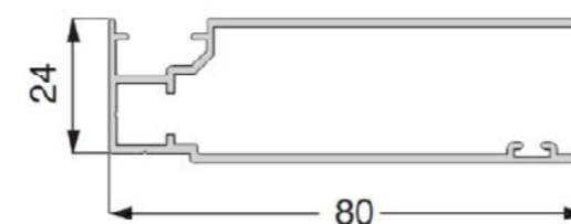
Side Channel
