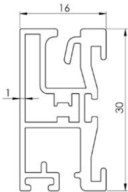
Bottom Bar (When Supplied with side channels)
