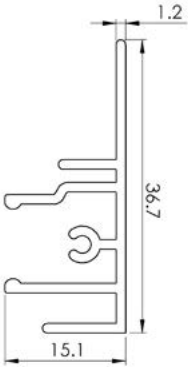
Side Channel (Back) Face Fix Application
