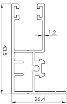
Side Channel (Front)
