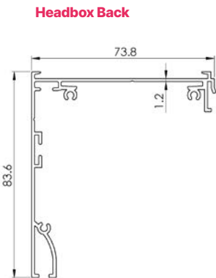
Headbox Back
