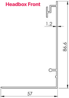
Headbox Front
