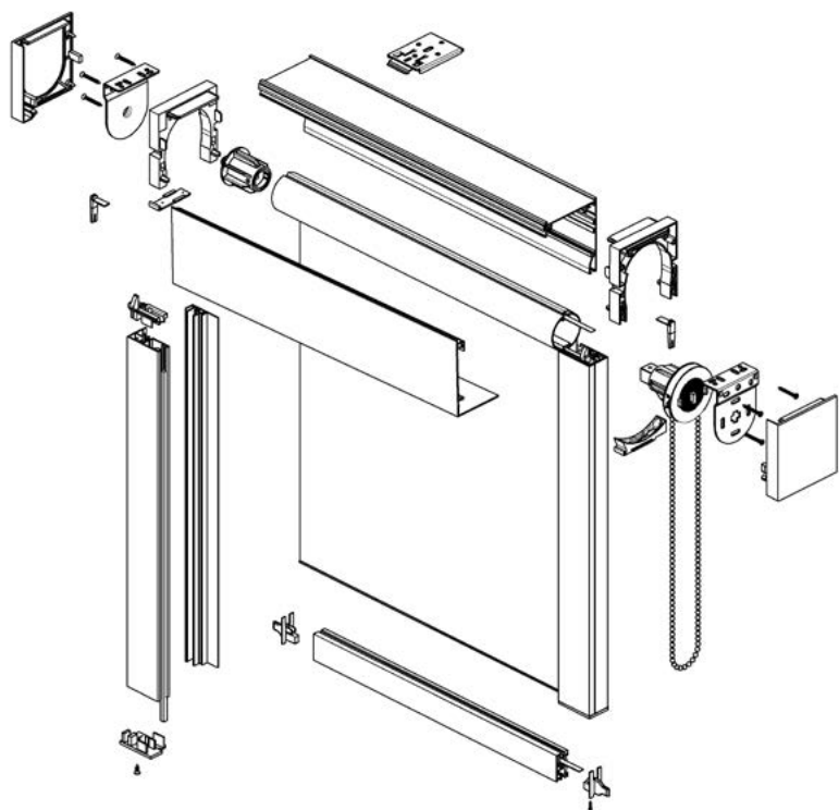
Exploded View
